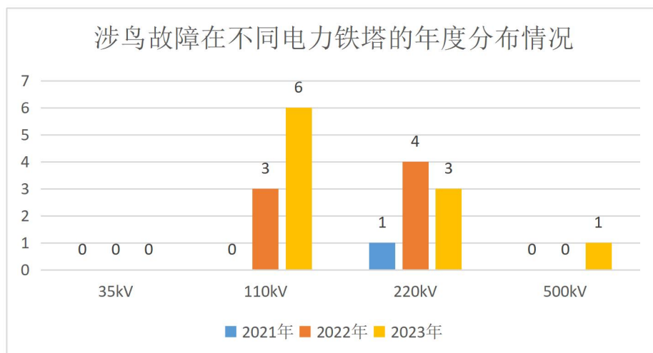
Annual distribution of bird-related incidents on different power towers
