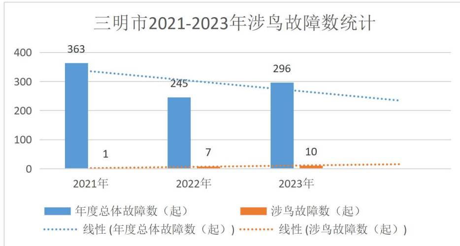
Statistics of bird-related incidents in Sanming from 2021 to 2023
