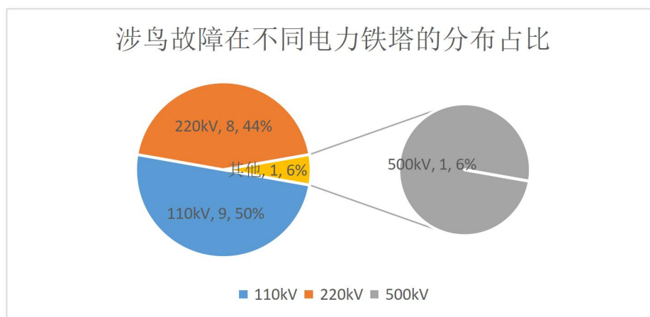
Distribution and proportion of bird-related incidents on different power towers
